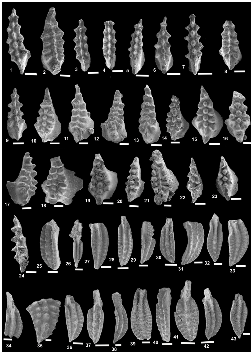
Figure 8 Conodonts from Yazdanshahr No2.section and sample numbers, respectively. 1, Icriodus eslaensis 26; 2, 8, I. arkonensis 45, 45; 3, 5, 24, I. alternatus costatus 24, 38, 55; 4, I. alternatus alternatus 46; 6, I. brevis 45; 7, 30, I. alternatus 28, 38; 9, I. brevis spicatus 34; 10, 12, 20, 21, 23, I. subterminus 56, 22, 25, 26, 33; 11, I. expansus 58; 13, I. difficilis 22; 14, I. orri 22; 15, 18, 19, I. excavatus 27, 36, 36; 16, I. alborzensis 26; 17, 22, Icriodus sp. 25, 45; 25, 42, Polygnathus sp. 36,36; 26, P. brevilamminus 33; 27, 31, 34, 36, P. webbi 24, 22, 44, 55; 28, 33, P. politus 26, 34; 29, 38, 40, P. xylus 22, 22, 44; 39, 43, P. pseudofoliatus 22, 26; 32, P. dubius 26; 35, Ancyrodella sp. 66; 37, Polygnathus alatus 22; 41, P. ovatinodosus 36. Scale bars = 100 \mu .
