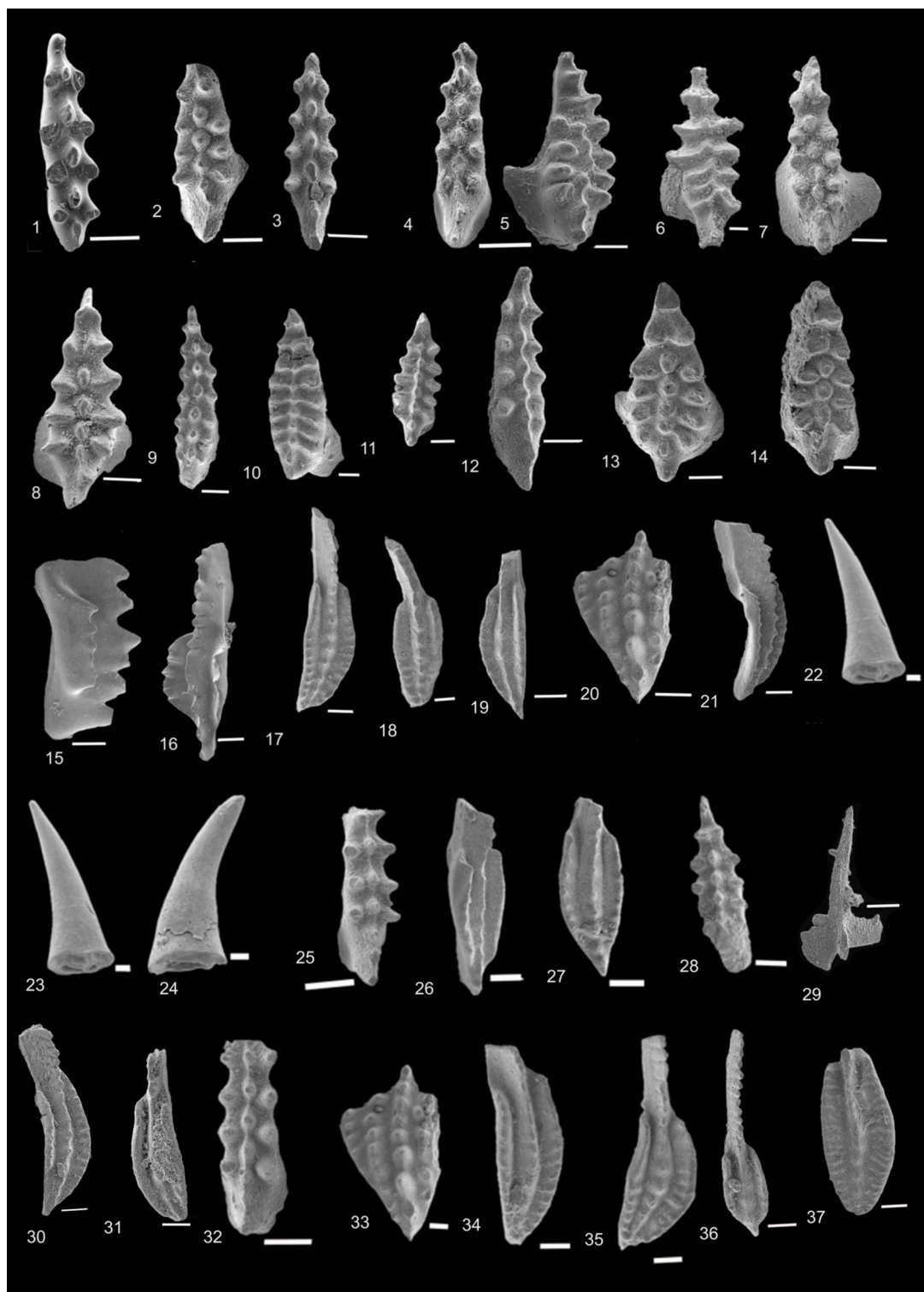
Figure 9 Conodonts from Yazdandshahr No.2 section and sample numbers, respectively. 1, 4, 9, Icriodus alternatus alternatus 46, 56, 46; 2, 7, 13, 14, I. subterminus 45, 30, 24; 3, I. alternatus costatus 46; 5, 12, 25, 28, 32, Icriodus sp. 36, 26, 28 22, 26; 6, 8, I. iowaensis 30, 36; 15, 16 Polygnathus breviamminis 42, 44; 17, 34, 35, 37, P. webbi 36, 42, 44, 38; 18, P. politus 28; 19, 20, 26, 31, P. decorsus 28, 34, 42, 48; 20, 33, Ancyrodella sp. 68, 66; 21, 30, Polygnathus xylus 48, 50; 22, 23, 24, Fish teeth 22, 22, 26; 27, Polygnathus sp 26; 29, Trichonodella sp. 50; 36, Polygnathus varcus 26. Scale bars = 100 \mu .
