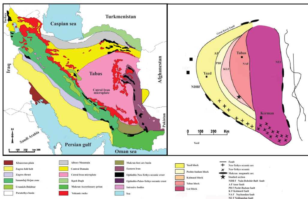
Figure 1 Structural units of Iran with location of the Yazdanshahr No.2 section (after Königshof et al. , 2017; Bahrami et al. , 2020).
