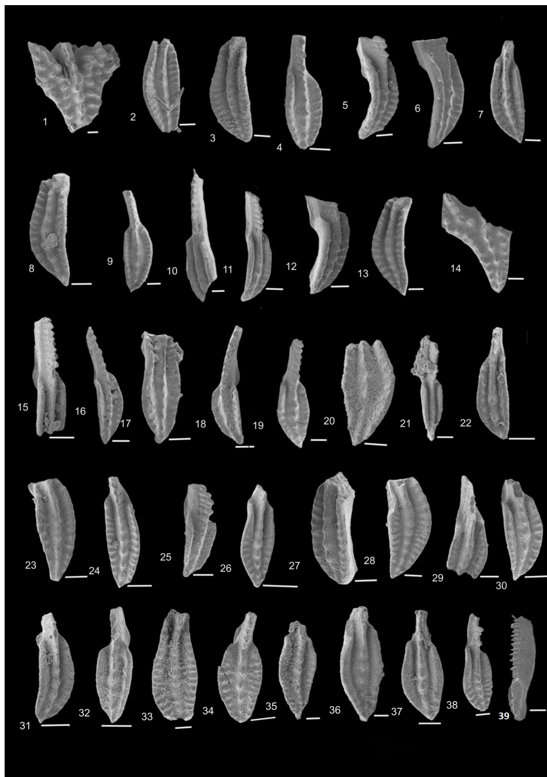
Figure 10 Conodonts from Yazdanshahr No. 2. section and sample numbers, respectively. 1, 14, Ancyrodella sp. 68, 66; 2, 3, 9, 12, 23, 29, 30, 38, Polygnathus webbi 36, 26, 40, 26, 32, 22, 46, 28; 4, 19, P. decorsus 40, 34; 5, 6, 8, 10, 13, 15, 25, P. xylus 25, 36, 36, 28, 22, 33, 26; 7, 33, P. dubius 24, 26; 11, 16, 24, 28, P. politus 28, 36, 40, 40; 17, 20, 36, 37, P. aequalis 44, 26, 42, 36; 18, P. timorensis 44; 21, P. brevilamminus 22; 22, 26, 32, P. alatus 30, 22, 43; 27, 31, Polygnathus sp. 28, 36; 4, P. ovatinodosus 44; 35, P. pseudofoliatus 46; 39, P. varcus 24. Scale bars = 100 \mu .
