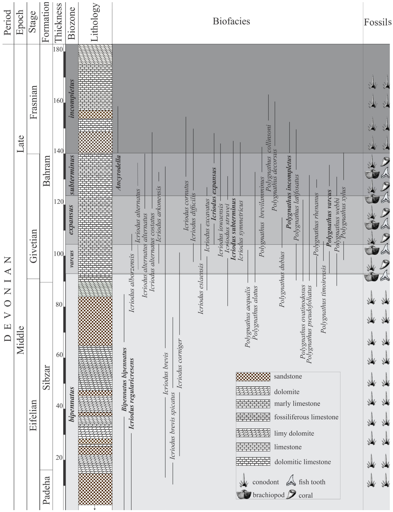
Figure 5 Biostratigraphic column of Yazdانشahr No.2 section.
