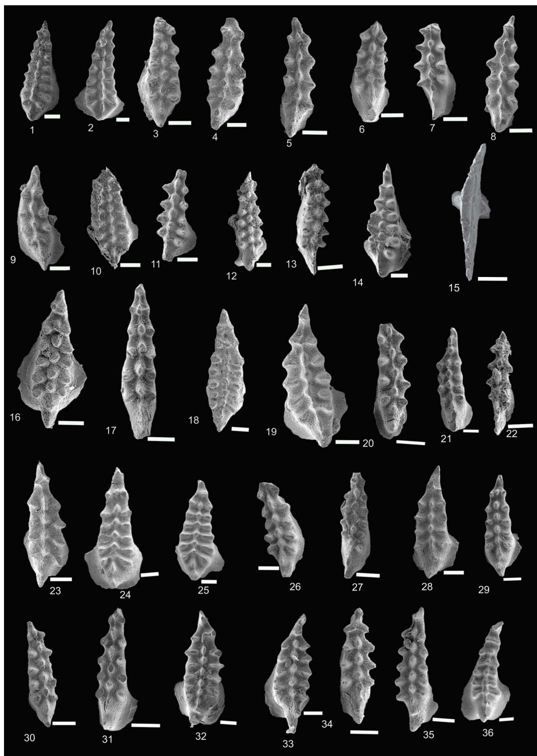
Figure 6 Conodonts from Yazdandshahr No.2 section and sample numbers, respectively. 1, 2, 10, 25, Icriodus symmetricus symmetricus 55, 52, 34, 45; 3, 4, 6, 8, I. eslaensis 37, 34, 25; 5, 13, 35, I. alternatus costatus 29, 33, 28; 7, 11, 21, 22, I. brevis 22, 29, 26, 25; 9, Icriodus sp. 38; 12, Icriodus cf. eslaensis 38; 14, I. subterminus 22; 15, Bipennatus bipennatus 18; 16, I. alborzensis 24; 17, 20, 31, I. alternatus alternatus 56, 36, 39; 18, 24, 32, I. arkonensis 30, 21, 21; 19, 23, 26, 29, 33, I. expansus 22, 20, 29, 33, 20; 27, 30, I. alternatus 47, 45; 28, I. symmetricus 61; 34, I. brevis brevis 56; 36, Icriodus corniger 25. Scale bars = 100 \mu
