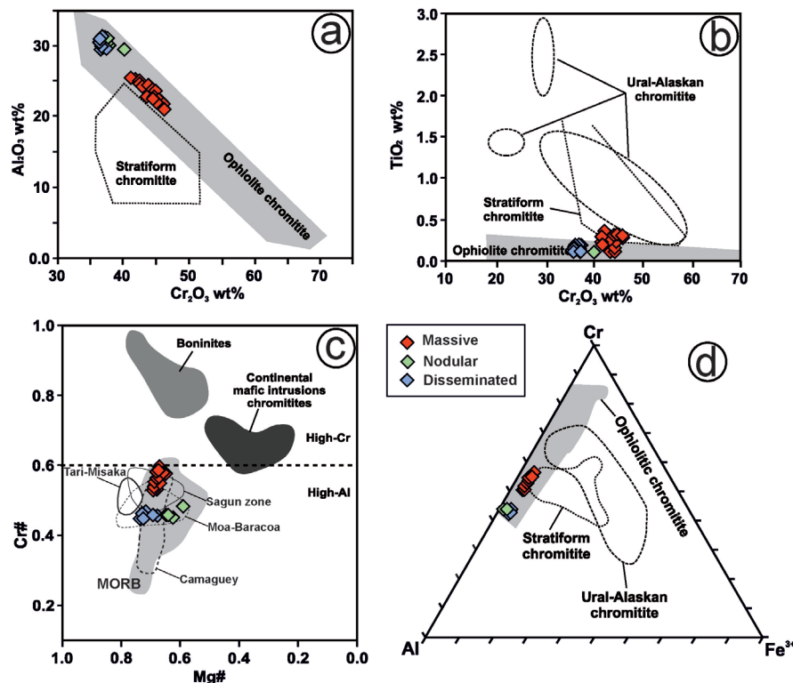
Figure 6 Chemistry of primary chromites from the Cerro Colorado chromitite as compared to chromite from various tectonic settings in terms of (a) Al_2O_3 vs. Cr_2O_3 , (b) TiO_2 vs Cr_2O_3 , (c) Cr# [ Cr/(Cr+Al) atomic ratio] vs Mg# [ Mg/(Mg+Fe) atomic ratio] and (d) Al-Cr- Fe^{3+} compositions. Data sources for chromian spinel of different tectonic settings are Bonavia et al. (1993), Kamenetsky et al. (2001) and Proenza et al. (2007). Legend is inset in the figure (note that semi-massive samples shown in Table 1 include also the nodular chromitite plotted in the figure).
