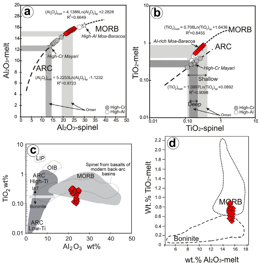
Figure 11 Al_2O_3 (a) and TiO_2 (b) contents of the melt in equilibrium with the Cerro Colorado high-Al chromite. The regression lines are from Zaccarini et al. (2011) using data on chromite-melt inclusions in MORB and arc lavas reported by Kamenetsky et al. (2001) and Rollinson (2008). The range of chromite and the calculated melt compositions from the shallow and deep Wadi Rajmi chromitites in Oman (Rollinson, 2008), and for high-Al and high-Cr chromitites from Mayarí-Baracoa ophiolitic belt in eastern Cuba (González-Jiménez et al. , 2011a) are shown for comparison. Only data of massive chromitite samples were used for computation. (c) Chemistry of chromite of massive chromitites forming the Cerro Colorado chromitite plot in terms of TiO_2 versus Al_2O_3 . Data sources for chromian spinel of different tectonic settings were obtained after Kamenetsky et al. (2001) and from the compilation of plots shown in Proenza et al. (2007). (d) TiO_2 and Al_2O_3 (wt. %) content of the melt calculated to be in equilibrium with chromite from the Cerro Colorado chromitite compared to the fields for chromites from boninites and MORB sources (after Pagé and Barnes, 2009).
