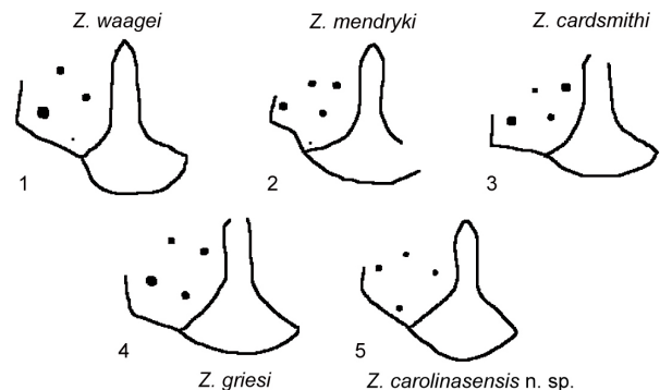
Figure 4. Hepatic and protogastric regions with the tubercles indicated by black dots of Zygastrocarcinus spp. The mesogastric region is also outlined. The drawing of Zygastrocarcinus waagei is based on Feldmann et al. (2008, fig. 1b), Z. mendryki based on Bishop (1982, fig. 3a, mirrored horizontally here), Z. cardsmithi based on Bishop (1986, fig. 2.2), and Z. griesi based on Bishop (1983, fig. 3d).
